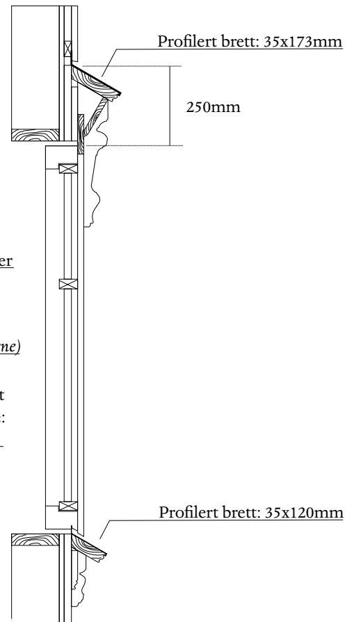
Brett, under 35x120mm
